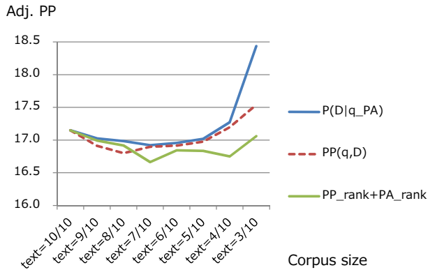
Figure 7: Adjusted perplexity on news navigation task.
